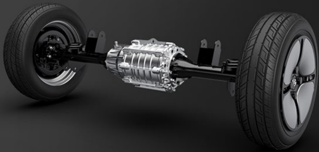
INTEGRATED MOTOR REAR DRIVE REAR SUSPENSION MECHANISM
